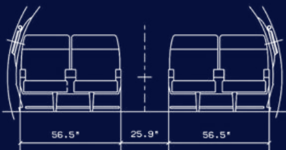
6 ABREAST CONSTANT SECTION
